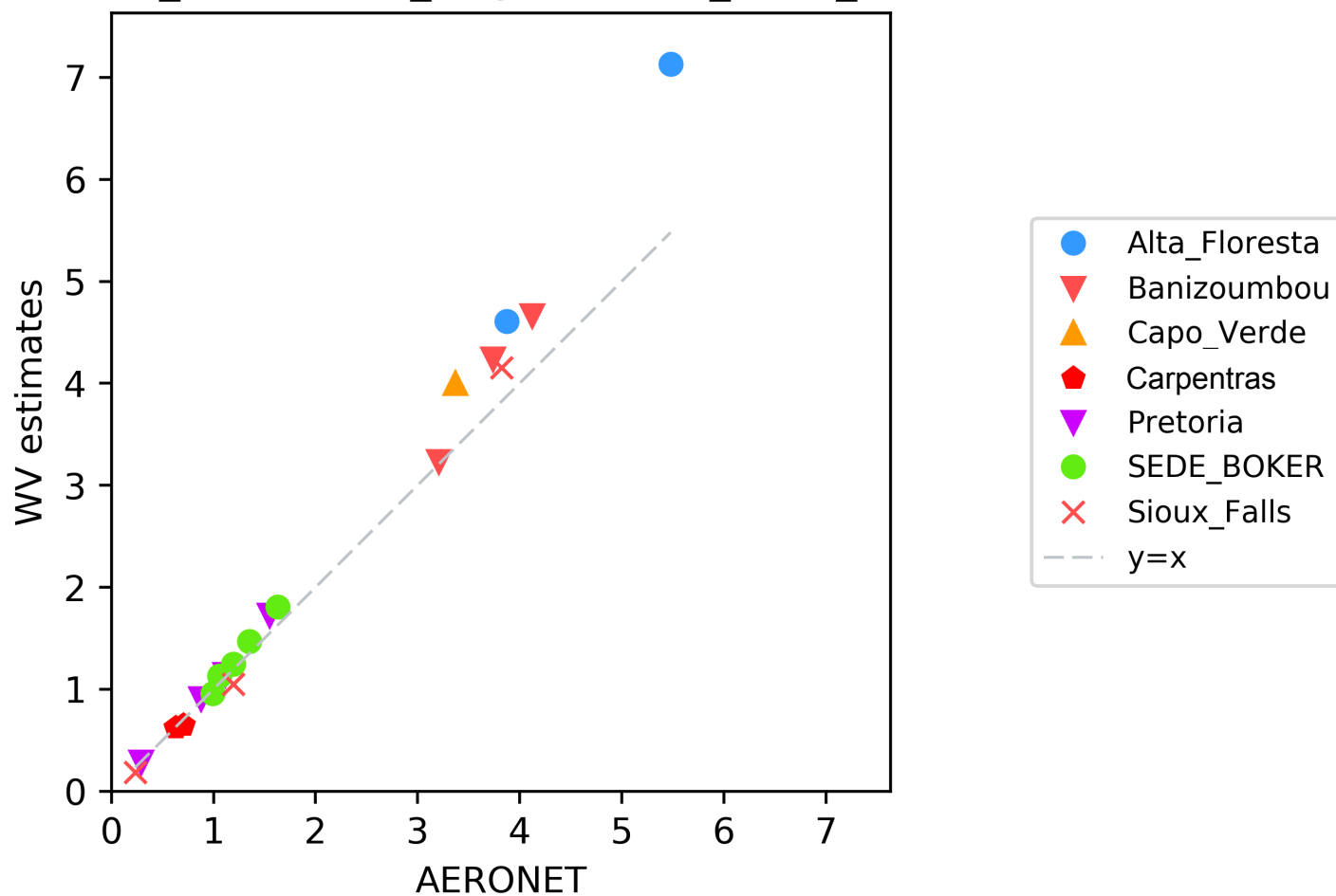
MACCS_WITHOUT_ADJACENCY_AND_SLOPE
