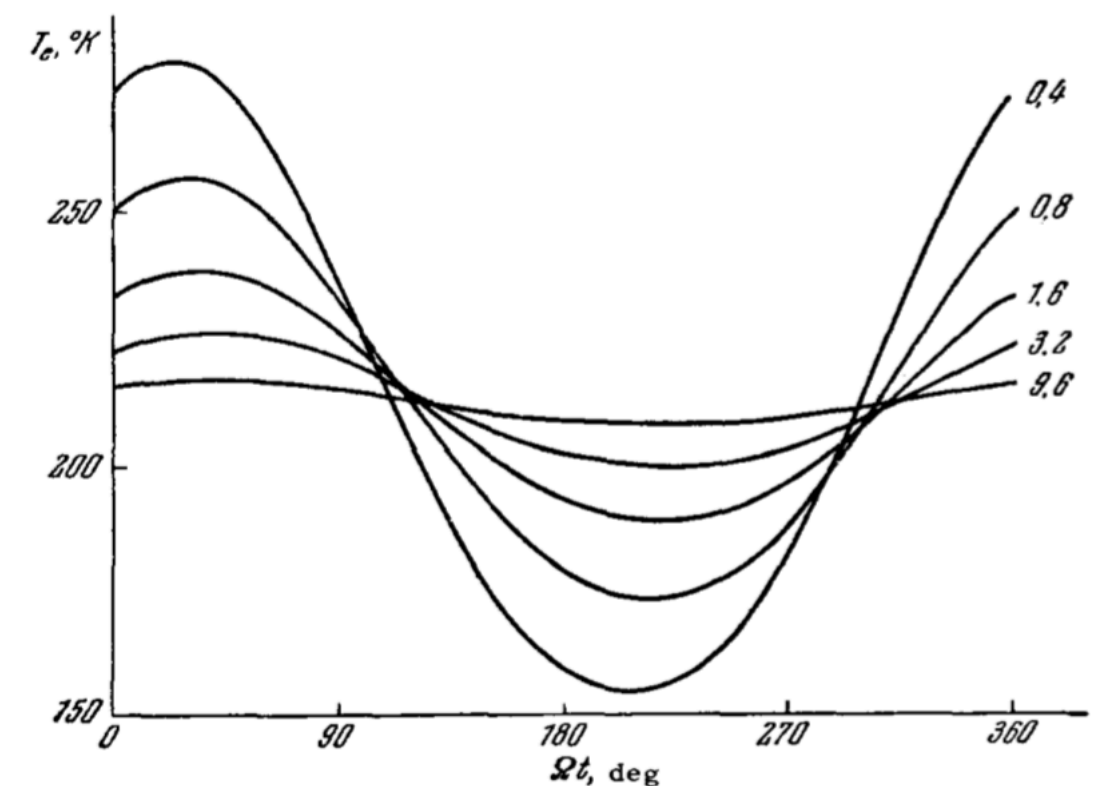
Model Simulations of Tb Averaged over the Moons Disk at Different Wavelength
