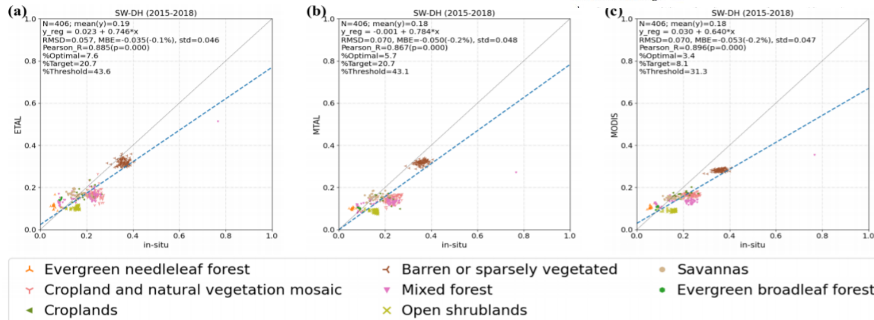
Figure 7. Accuracy assessment of (a) ETAL, (b) MTAL-R/NRT and (c) MODIS surface albedo satellite products versus ground measurements coming from GBOV, AMMA and BSRN stations during the 1 January 2015–31 December 2018 period. Only those dates that provided concomitant data for all three
